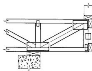
Load-Bearing Wall Cantilever Special Engineering Required
