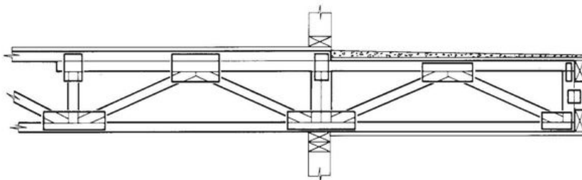
Dropped Chord Balcony Cantilever Special Engineering Required
