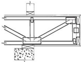
Balcony Cantilever Special Engineering Required
